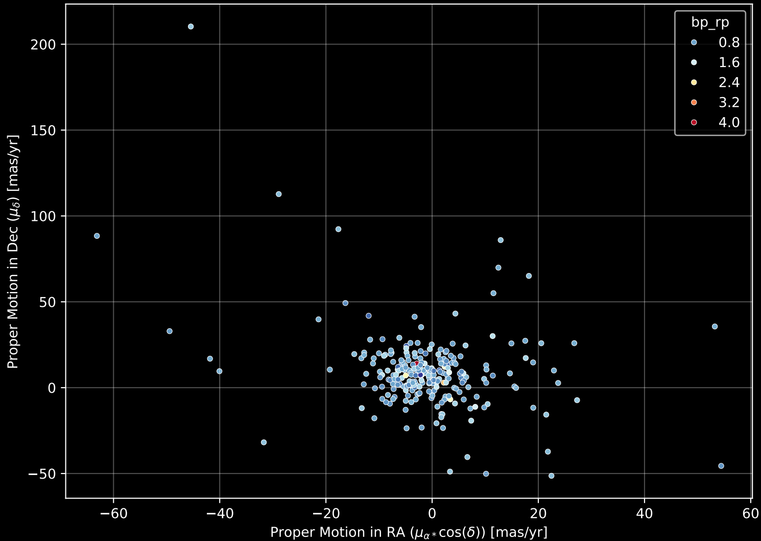
GALAH DR4 Field: [7163] Proper Motion Diagram (n= 264)
