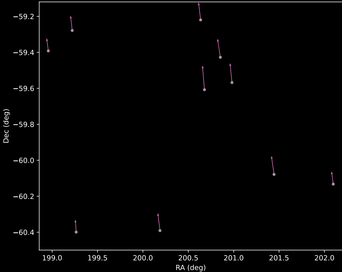
GALAH DR4 Cluster 12 Proper Motion Vectors (n=10)
