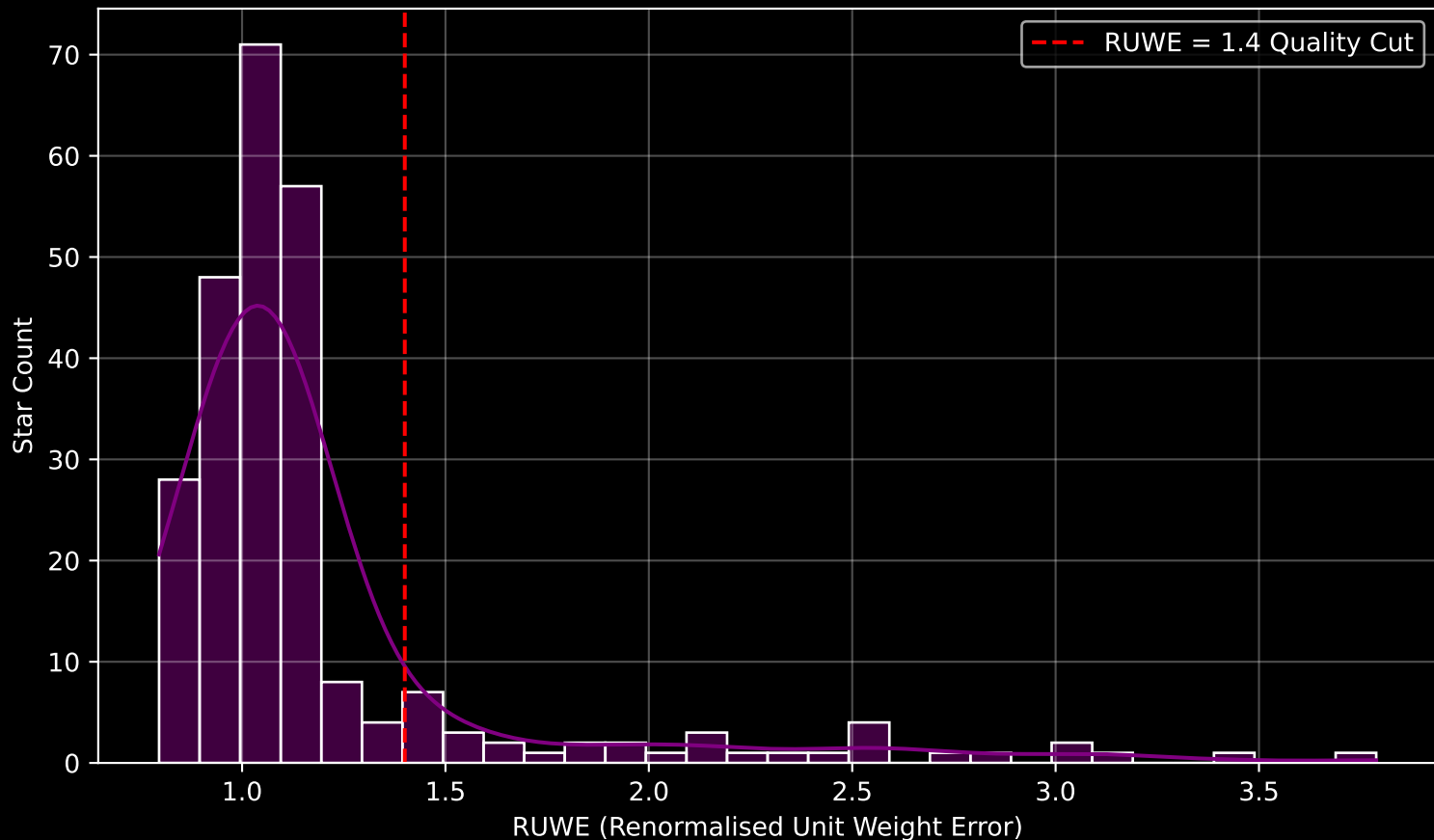
GALAH DR4 Field [7163] RUWE Distribution (n= 251)
