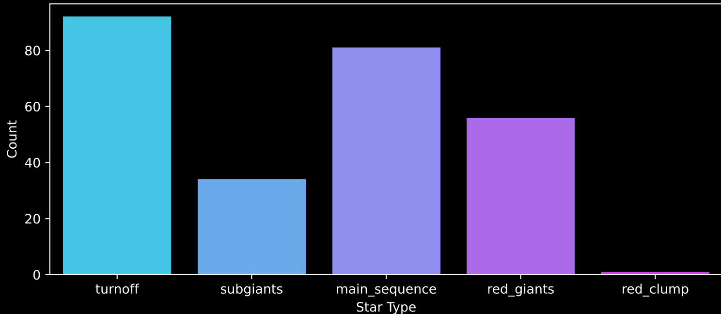
GALAH DR4 Field: [7163] Count plot of Star Type
